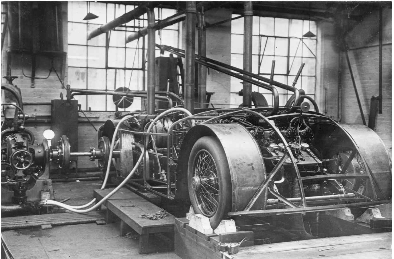
Sunbeam 1000hp under construction.
